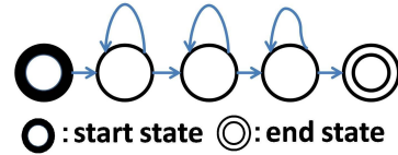
図 9 left-to-right HMM Fig. 9 A left-to-right HMM.
