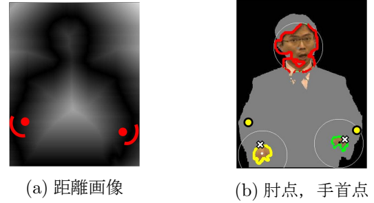
図 8 肘点, 手首点の検出 Fig. 8 Detection of elbow points and wrist points.
